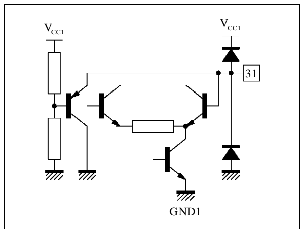
Figure 28 : Pin 31 - BCL
