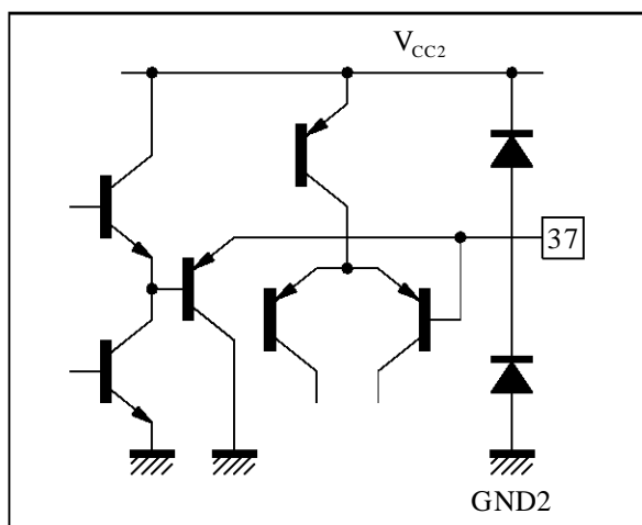
Figure 34 : Pin 37 - LFB/SC
