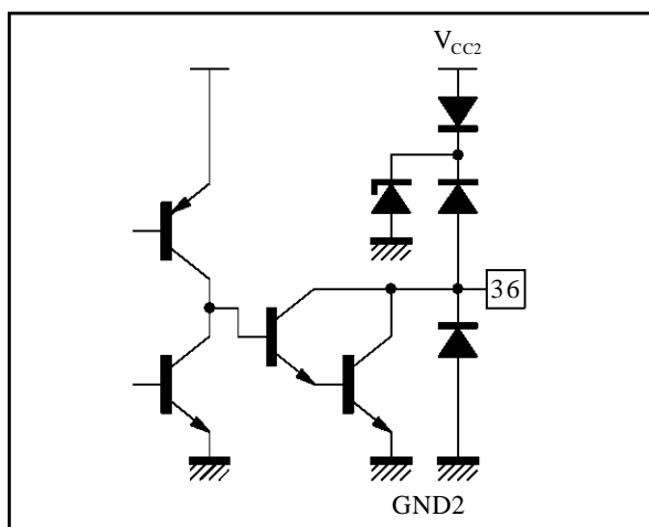
Figure 33 : Pin 36 - HOUT
